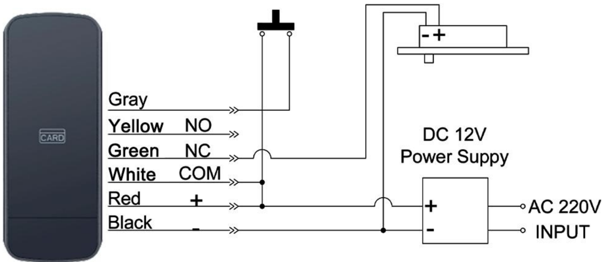
Electric Bolt Lock or Magnetic lock
