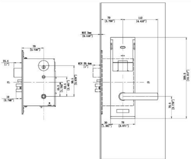
ANSI lockcase
