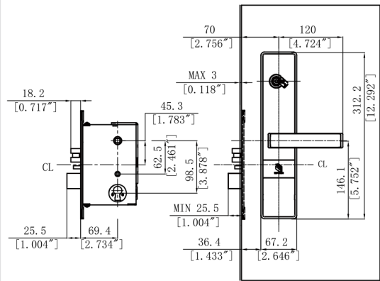
ANSI Lockcase
